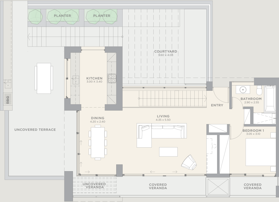
Lower Floor
