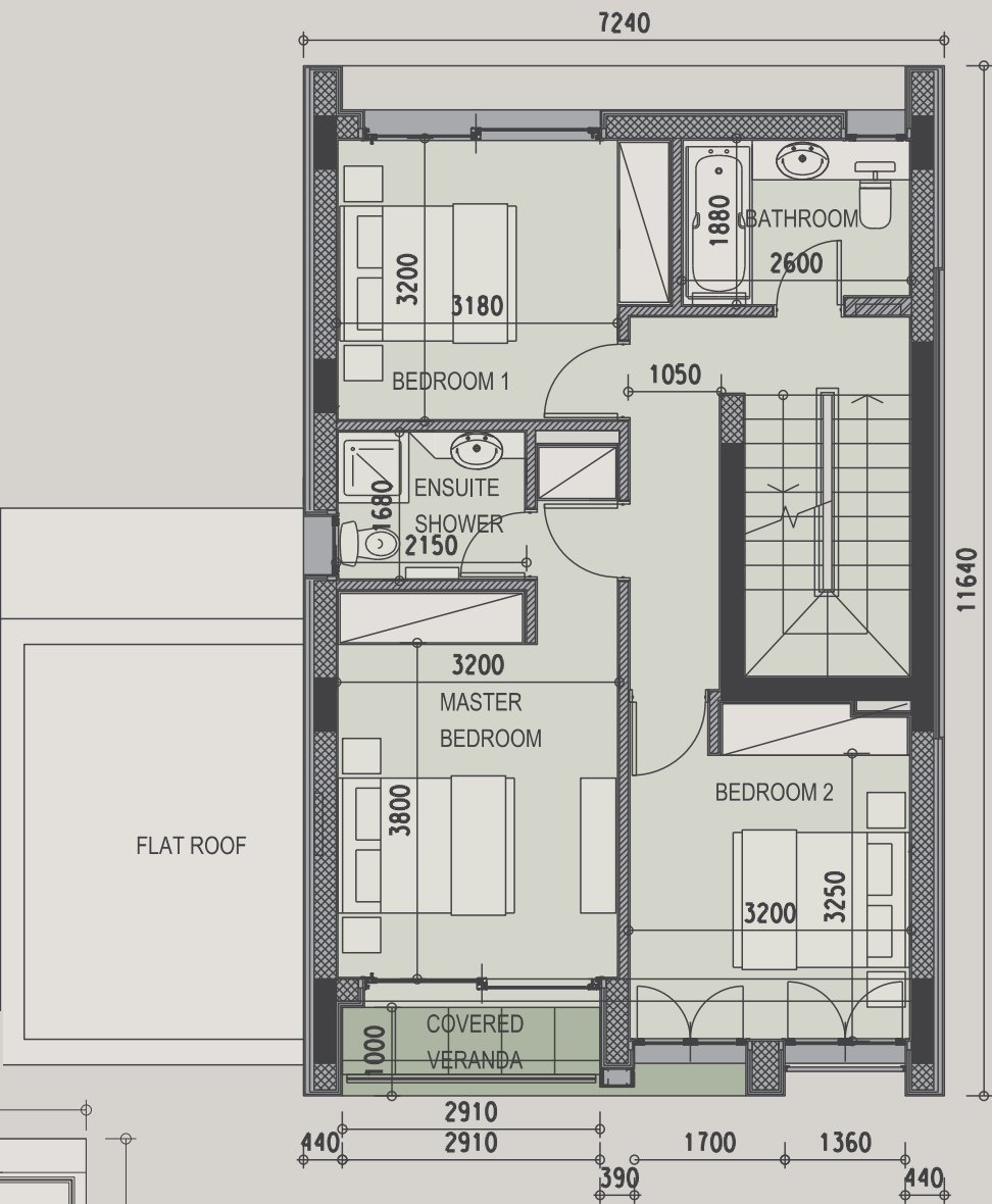
FIRST FLOOR
