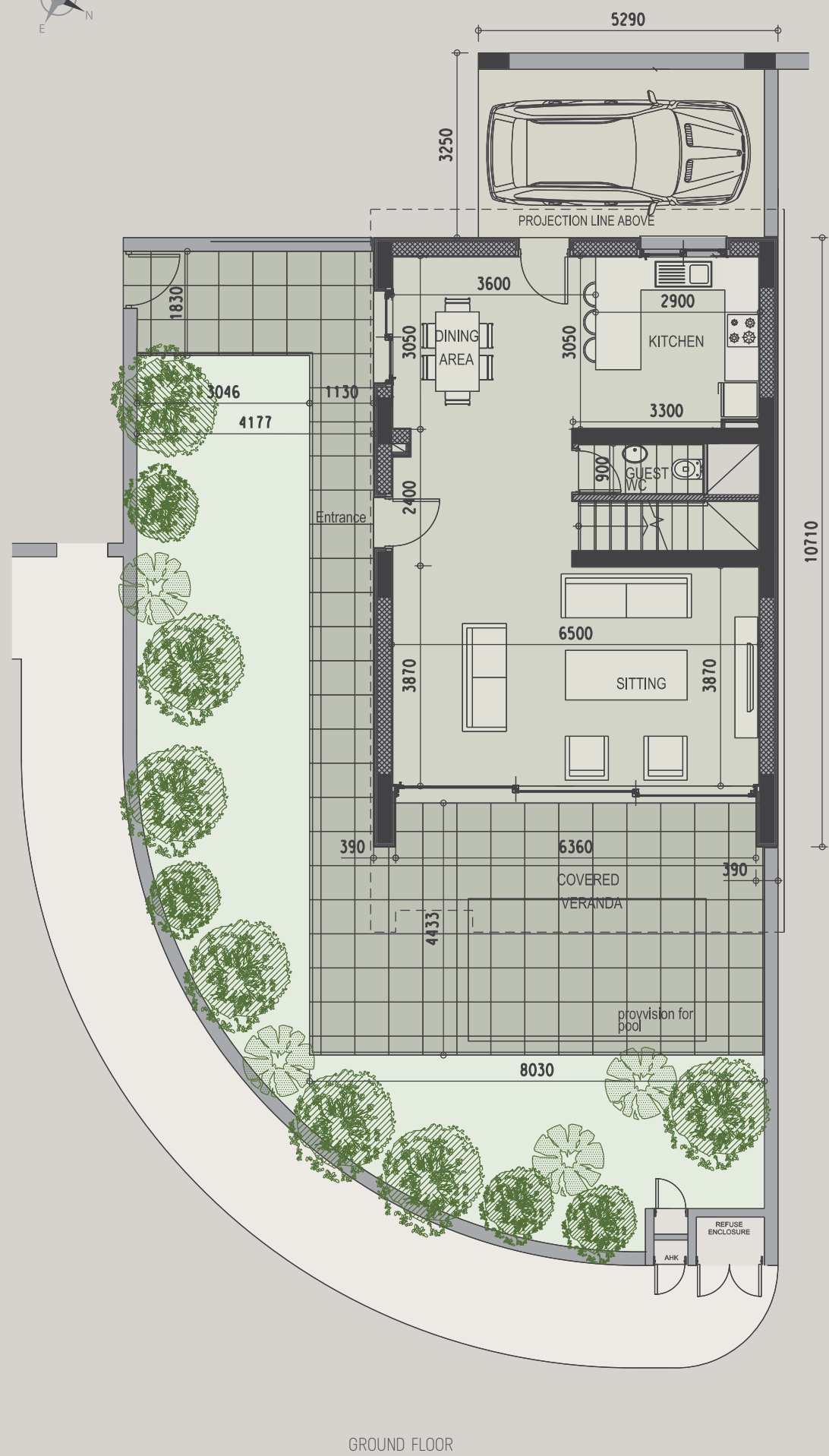
GROUND FLOOR
