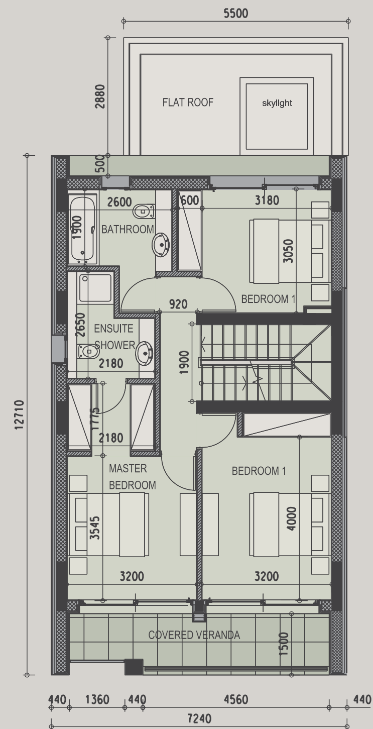
FIRST FLOOR
